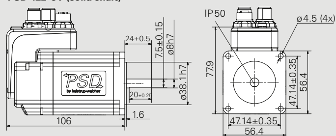
PSD 432-8/14H (hollow shaft, 2 and 4 Nm)
